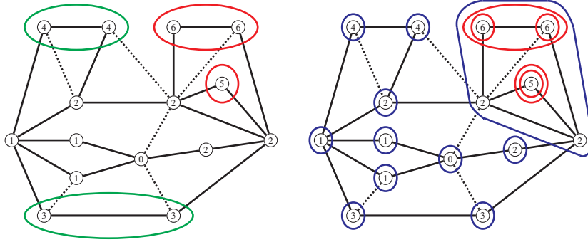
Figure 13.5 Left: The nicer ear-decomposition from Figure 13.4 (according to Theorem 13.17). The red sets are the elements of \mathcal{B} ; the green sets are the elements of \mathcal{I} \setminus \mathcal{B} . Right: The cuts in the proof of Theorem 13.18. The partition \mathcal{U} is shown in blue.
