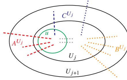
Figure 11.7 The figure shows an example of the sets u , U_j , and U_{j+1} together with the edges in \delta(u) and in \delta(U_j) . The edges in \delta(u) \cap \delta(U_j) are dashed, while other edges are dotted. The colors of the edges indicate the \varepsilon_{\text{partition}} -degree partition of \delta(U_j) into A^{U_j} (red), B^{U_j} (orange), and C^{U_j} (blue).
