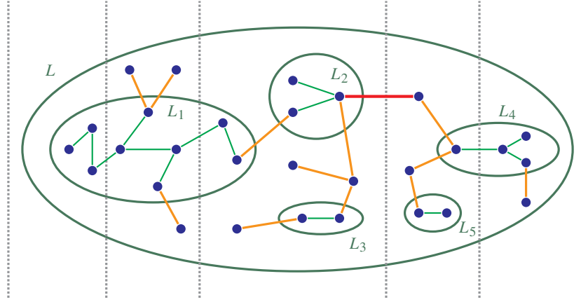
Figure 15.5 Illustration of the construction of S_L in the proof of Lemma 15.16. Narrow cuts are shown as gray dotted lines. The dark-green ellipses show a set L in the laminar family \mathcal{V} \cup \mathcal{L} and its maximal subsets L_1, \dots, L_5 \in \mathcal{L} . The light-green edges are the edges of the trees (L_1, S_{L_1}), \dots, (L_5, S_{L_5}) . The edges added to S_{L_1} \cup \dots \cup S_{L_5} to obtain S'_L are shown in orange. Finally, we add the edge drawn in red, which completes S'_L to the tree S_L with the desired properties.
