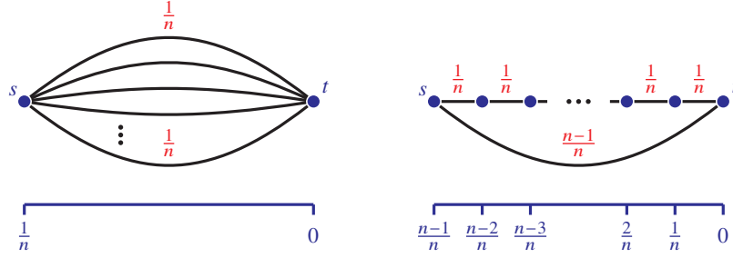
Figure 5.4 Two graphs G = (V, E) , both with n edges and with \lambda_e = 1 for all e \in E . The electrical s - t -flow of value 1 is shown in red above the edges, flowing from left to right. A corresponding potential \pi is shown in blue below. The effective resistance of every edge is \frac{1}{n} on the left and \frac{n-1}{n} on the right; this is the probability that an edge belongs to a random spanning tree in the uniform distribution.
