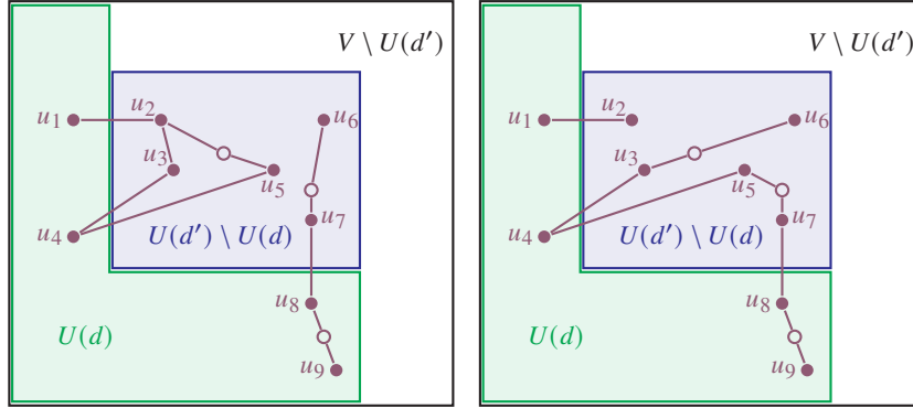
Figure 16.8 Illustration of two parallel arcs (d, d') in the digraph (D, A) . In this example, the boxed set U(d') is shown in green and blue; its terminal pairs in T(d') are \{u_1, u_2\} and \{u_6, u_9\} . The boxed set U(d) is shown in green, and its terminal pairs in T(d) are \{u_1, u_1\} , \{u_4, u_4\} , and \{u_8, u_9\} . The left and the right part of the figure show two different ways of extending the same solution to the MULTI-PATH TSP instance (G[U(d)], c, T(d)) to a solution to the MULTI-PATH TSP instance (G[U(d')], c, T(d')) . These two different extensions can be obtained by considering two different arcs from d to d' , corresponding to two different multi-sets of border protocols for U(d) in G[U(d')] . The solution on the left is obtained by considering the multi-set of border protocols that consists of u_1, u_1, u_2, u_3, u_4, u_4, u_5, u_2 and u_6, u_7, u_8, u_9 , then computing a solution to the induced instance with vertex set U(d') \setminus U(d) and terminal pairs \{u_2, u_3\} , \{u_5, u_2\} , \{u_6, u_7\} , and applying Lemma 16.17. The solution on the right is obtained by considering the multi-set of border protocols that consists of u_1, u_1, u_2, u_2 and u_6, u_3, u_4, u_4, u_5, u_7, u_8, u_9 , then computing a solution to the induced instance with vertex set U(d') \setminus U(d) and terminal pairs \{u_2, u_2\} , \{u_6, u_3\} , \{u_5, u_7\} , and applying Lemma 16.17.
