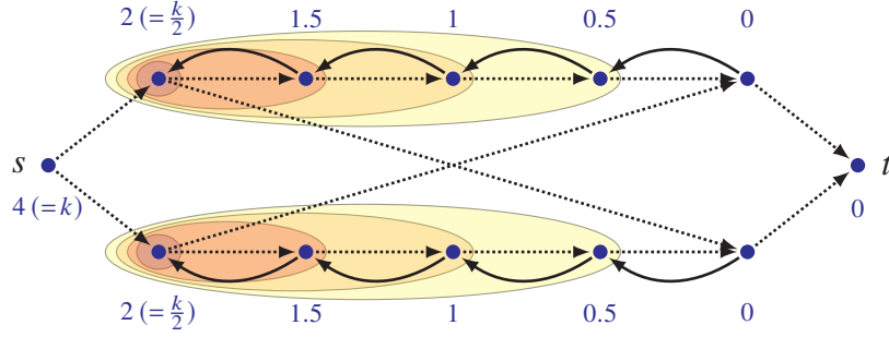
Figure 9.3 Example by Friggstad, Gupta, and Singh [2016] with integrality ratio approaching 2 as the number of vertices increases. Setting x_e := \frac{1}{2} for all shown edges defines a feasible solution to (9.1). If the 2k curved edges have cost 1 and the dotted edges have cost 0, we have \text{LP} = c(x) = k , but any s - t -tour costs at least 2k - 1 . (In the figure, k = 4 .) Setting y_U = \frac{1}{2} for the vertex sets U indicated by the ellipses and a_v as shown in blue defines an optimum solution to the dual LP (9.3). This dual solution has strongly laminar support. This picture is taken from Köhne, Traub, and Vygen [2020] (with permission from Springer Nature).
