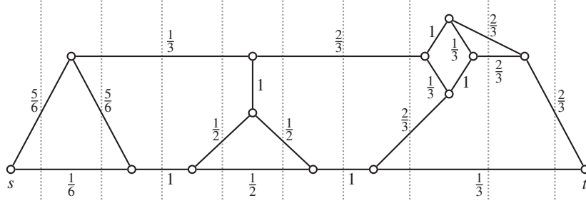
Figure 14.3 An LP solution (numbers in black) to a PATH TSP instance and the narrow cuts (gray dotted lines), which form a chain.
