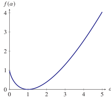
Figure 5.2 The function f in Lemma 5.6.
