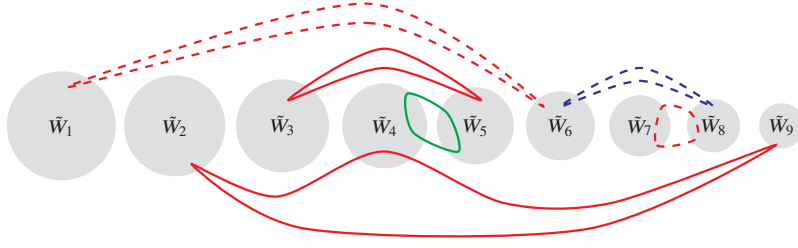
Figure 6.4 An illustration of Step (6) in the first iteration of Svensson's algorithm. The edge set F is shown in red (solid and dashed). First, the component Z with vertex set \tilde{W}_7 \cup \tilde{W}_8 and \text{ind}(Z) = 7 is considered. We may find the blue circuit C with |E(C)| \leq \text{slack}(\tilde{W}_7, \tilde{H}) . After adding E(C) to X , the component Z with vertex set \tilde{W}_3 \cup \tilde{W}_5 and \text{ind}(Z) = 3 is considered next. Then we may find the green circuit C' with |E(C')| \leq \text{slack}(\tilde{W}_3, \tilde{H}) . Then E(C') is added to X , and now (V, H \dot{\cup} F \dot{\cup} X) has two connected components. The component Z with vertex set \tilde{W}_2 \cup \tilde{W}_3 \cup \tilde{W}_4 \cup \tilde{W}_5 \cup \tilde{W}_9 and \text{ind}(Z) = 2 is considered next. Suppose there is no circuit C'' connecting it to the rest and with |E(C'')| \leq \text{slack}(\tilde{W}_2, \tilde{H}) . Then the edges drawn as solid curves are added to H , concluding the first iteration. This picture is taken from Traub and Vygen [2022].
