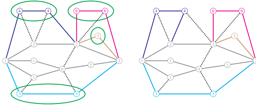
Figure 13.4 Left: A graph G with a nice ear-decomposition. The short ears are highlighted in color, and the elements of \mathcal{I} are the green sets. Right: A nicer ear-decomposition, in which the spanning subgraph that contains only the edges of the short ears has fewer connected components (five instead of six). Only ear P_4 has been modified here.
