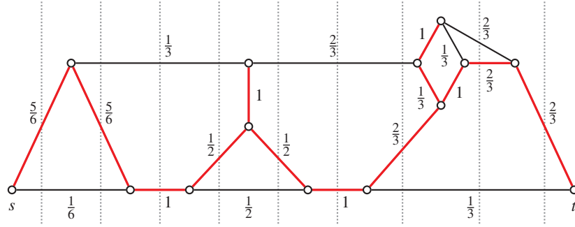
Figure 14.4 A Gao tree (red, thick) for the LP solution (numbers in black) of Figure 14.3; again, the narrow cuts are shown by gray dotted lines. The Gao tree contains exactly one edge in each narrow cut.
