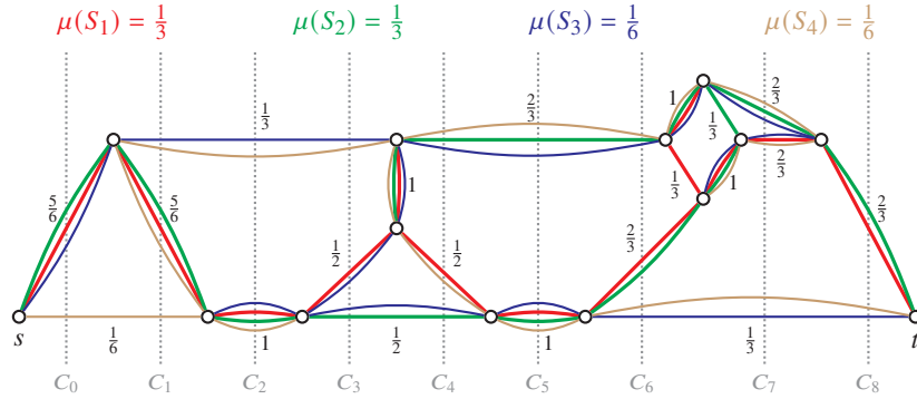
Figure 15.4 Continuing the example from Figure 14.4, the picture shows a decomposition of the LP solution x^* (black numbers) into spanning trees, satisfying the properties of Theorem 15.13. Here x^* = \frac{1}{3}\chi^{S_1} + \frac{1}{3}\chi^{S_2} + \frac{1}{6}\chi^{S_3} + \frac{1}{6}\chi^{S_4} . The trees S_1, S_2, S_3, S_4 are shown in red, green, blue, and brown, respectively. As required, S_1 is a Gao tree, and S_2 has only one edge in each of the cuts C_0, C_1, C_2, C_3, C_8 with value less than \frac{5}{3} .
