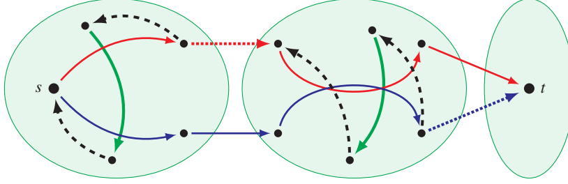
Figure 9.9 Construction of the walk Q . The s - t -paths P_1 (red) and P_2 (blue) are shown with solid and dotted lines. The vertex sets V_1, \dots, V_l of the strongly connected components are indicated by the green ellipses (here l = 3 , and V_3 contains only t ). The thick green curves illustrate the nice paths P_{u_i^*, v_i^*} that we include in the backbone. The red and blue solid parts of the paths P_i are those that are used for the backbone; the dotted edges are omitted. The dashed black arrows indicate the paths that we add.
