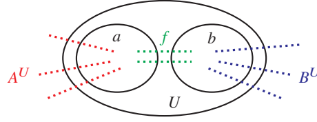
Figure 11.9 The figure illustrates the choice of the \varepsilon_{\text{partition}} -degree partition for a triangle U with children a, b \in \mathcal{H} . The green edges form the edge bundle f = \{a, b\} . We have U = a \cup b and x(A^U) \approx x(B^U) \approx x_f \approx 1 .
