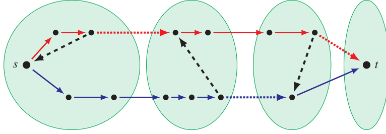
Figure 9.5 Construction of the s - t -walk P in the proof of Theorem 9.11. The s - t -walks P_1 and P_2 are shown with solid and dotted lines. (Here, P_1 is the red walk at the top, and P_2 is shown in blue at the bottom.) The vertex sets V_1, \dots, V_l of the strongly connected components are indicated by the green ellipses. The red and blue solid edges of the walks P_1 and P_2 are those that are used in the walk P . The dashed black arrows indicate the paths within the sets V_i that we add. This picture is taken from Köhne, Traub, and Vygen [2020] (with permission from Springer Nature).
