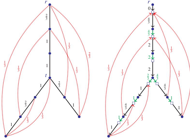
Figure 12.5 Example for constructing a cheap circulation. Left: an LP solution x and a possible DFS tree (rooted at r ) as computed in Step (2) of Algorithm 12.9, shown by the black solid edges. Right: the circulation f' . In this case, there is one green edge carrying less than one unit of flow; this will be compensated by f'' .
