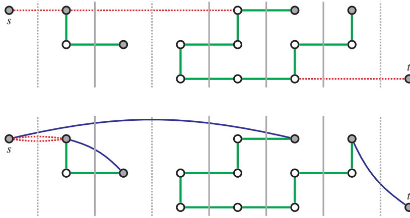
Figure 15.6 Top: The spanning tree (V, S) from Figure 15.3. Again, the narrow cuts are those shown in grey (dotted and solid). The lonely edges are dotted and red. For each lonely edge, there is one narrow cut (dotted) in which this is the only edge of S (other narrow cuts are shown as solid lines). Removing the lonely edges from S results in a forest F_S (green). Filled circles show vertices in T \triangle \text{odd}(F_S) , where T = \{s, t\} .
