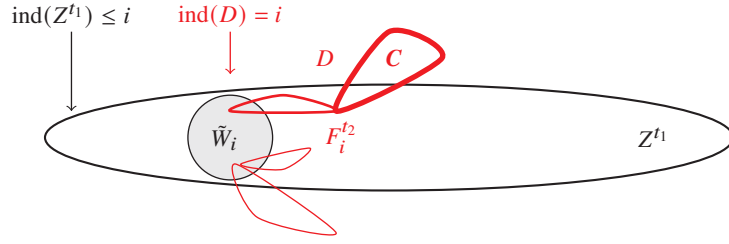
Figure 6.5 Proof of Lemma 6.15: An example of the graph F_i^{t_2} is shown in red. The circuit C contains an edge of \delta(V(Z^{t_1})) , and D is the connected component containing C . This picture is taken from Traub and Vygen [2022].
