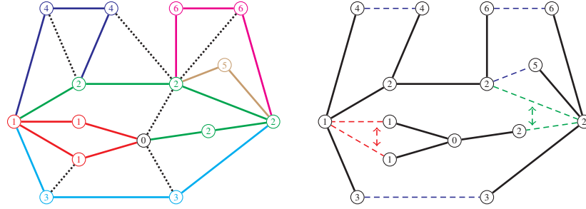
Figure 13.1 Left: A graph G with an open ear-decomposition. The ears P_1, \dots, P_6 have distinct colors; moreover, the internal vertices of the i -th ear are labelled i . The ears P_7, \dots, P_{12} are trivial; each consists of a single dotted edge. The ears P_1 and P_5 are even; the other ears are odd. The ears P_3, P_4, P_5 , and P_6 are short and pendant. Right: Trivial ears are deleted, and a removable pairing (R, \mathcal{P}) with |R| = 8 and |\mathcal{P}| = 2 as in the proof of Theorem 13.4 is shown; the dashed edges are removable, and the arrows indicate the two pairs.
