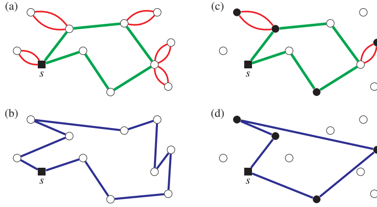
Figure 17.3 In (a), we see a master route solution with a master route (green) and connections of the other customers to that master route (red). In (b), the corresponding Hamiltonian circuit C is shown. In (d), we skip the inactive customers in C and obtain the circuit C_A on the set A of active customers (filled). In (c), the upper bound on c(C_A) obtained by the master route solution is illustrated.
