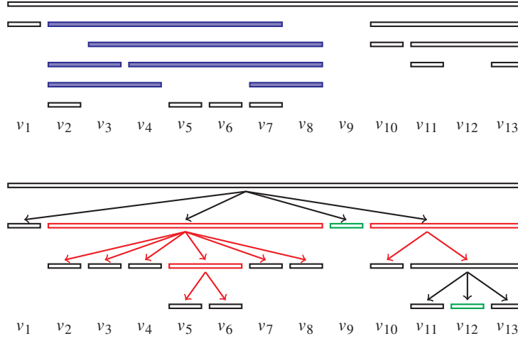
Figure 10.2 Top: The almost laminar family \mathcal{L} of the \eta -mincuts that are not irrelevant could look like this. Each set is shown as a horizontal bar representing the interval. Here there is only one nontrivial component, formed by subsets of \{v_2, \dots, v_8\} , shown as blue-filled bars. Bottom: The hierarchy \mathcal{H} corresponding to \mathcal{L} . The parent-child relation is shown by arrows. This hierarchy contains three polygons, shown in red. The polygon corresponding to the nontrivial component is \{v_2, \dots, v_8\} ; its atoms are \{v_2\} , \{v_3\} , \{v_4\} , \{v_5, v_6\} , \{v_7\} , and \{v_8\} . The two green singletons are irrelevant but still part of the hierarchy.
