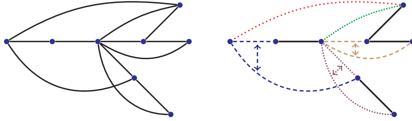
Figure 12.1 A 2-connected graph (left) and a removable pairing (right: dashed and dotted edges are removable; colors and arrows indicate pairs).
