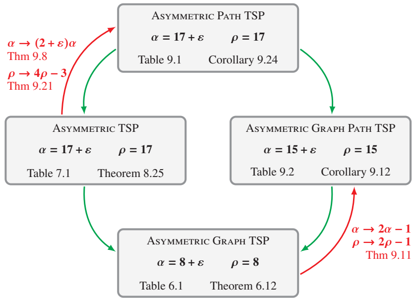
Figure 18.1 Approximation ratios ( \alpha ) and upper bounds on integrality ratios ( \rho ) for asymmetric traveling salesman problems: the state of the art. An arrow from one problem to another means an approximation or integrality ratio bound for the former implies an approximation or integrality ratio bound for the latter (the same by a trivial reduction for the green arcs without labels). The only known lower bound on the integrality ratio of all these problems is 2 (Theorem 3.18).
