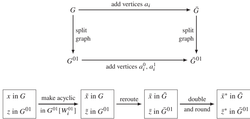
Figure 8.5 Overview of the different graphs and circulations occurring in the subtour cover algorithm. We start with the circulation x in G stemming from the strongly laminar ASYMMETRIC TSP instance (G, \mathcal{L}, x, y) . We map x to a circulation z in the split graph G^{01} and perform three steps, ending with an integral circulation \bar{z}^* in \bar{G}^{01} . This corresponds to an integral circulation \bar{x}^* in \bar{G} , which we will map back to G in the final step of the subtour cover algorithm. A similar picture appeared in Traub and Vygen [2022].
