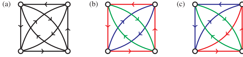
Figure 3.3 Decomposing a solution to (3.1) into circuits in an arbitrary way may not yield a feasible solution to (3.6), as this example (taken from Henke [2018]) shows. In (a) we see the support graph of a solution to (3.1), where each of the eight edges has value \frac{1}{2} . The pictures (b) and (c) show two decompositions of this circulation into flows on circuits; each of the circuits has value \frac{1}{2} . The decomposition in (c) is a feasible solution to (3.6), but the one in (b) is not.
