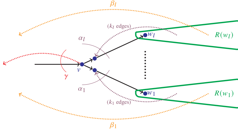
Figure 12.6 Illustrating \alpha_i, \beta_i ( i = 1, \dots, l ), and \gamma in the proof of Lemma 12.10. The edge set B_v consists of the violet dotted edges entering v : the k_i non-tree edges from R(w_i) to v for i = 1, \dots, l .
