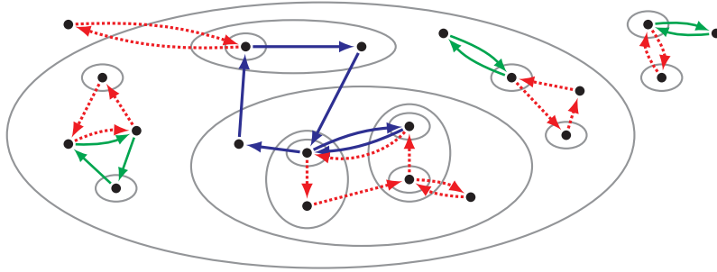
Figure 7.9 Example of a vertebrate pair (I, B) , a local Eulerian edge set H , and a subtour cover for (I, B, H) . The laminar family \mathcal{L} of \mathcal{I} is shown in gray, and the backbone B is shown in blue. The edge set H is shown in green, and a subtour cover consists of the dotted red edges.
