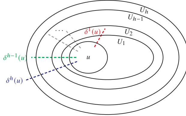
Figure 11.5 Illustration of the partition of \delta^\uparrow(u) , shown as dashed edges, into the sets \delta^j(u) for j \in \{1, \dots, h\} .
