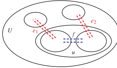
Figure 11.12 Illustration of the situation in which we choose the reduction events of the half-edge bundles e_1 and e_2 (shown in red) to be identical. By increasing the slack on the edge bundle f = \delta^{\rightarrow}(u) (shown in blue), we can simultaneously compensate for the reduction on both e_1 and e_2 .
