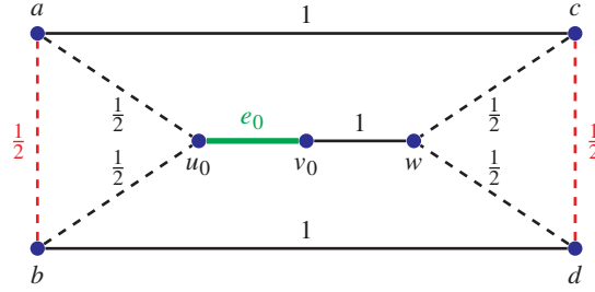
Figure 11.2 An example in which there exist edges e for which the probability that both top cuts of e are simultaneously even is zero. We have x_e = \frac{1}{2} for each dashed edge e and x_e = 1 for each solid edge e . Suppose the optimum tour visits the vertices a, b, w, c, d, u_0, v_0 in this order. Then the hierarchy consists only of singleton cuts and the set V \setminus \{u_0, v_0\} . Every spanning tree that is sampled with positive probability contains the edges \{a, c\} , \{v_0, w\} , \{b, d\} . Moreover, it contains precisely one of the edges \{a, u_0\} and \{b, u_0\} (since it must connect u_0 and does not contain e_0 ) and precisely one of the edges \{c, w\} and \{d, w\} . Thus, for the two red edges, the top cuts – which are \{a\} and \{b\} for the edge \{a, b\} and \{c\} and \{d\} for the edge \{c, d\} – are simultaneously even with probability zero.
