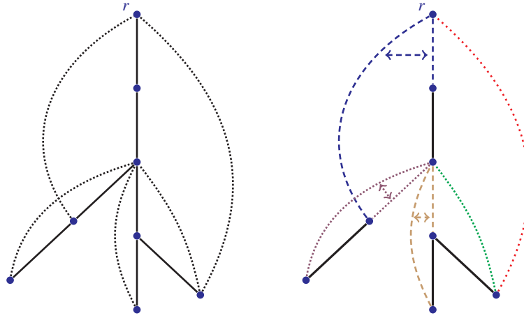
Figure 12.3 A 2-connected graph with a DFS tree rooted at r (left: solid edges) and a removable pairing resulting from the construction in Lemma 12.5 (right: dashed and dotted edges are removable; colors and arrows indicate pairs).
