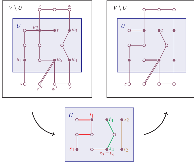
Figure 16.6 On the top left, we see a MULTI-PATH TSP instance \mathcal{I} with vertex set V , a terminal pair \{s, t\} , an \{s, t\} -tour, and a subset U of V . Other edges of this instance are not shown. If W is the sequence of vertices that we get when traversing this \{s, t\} -tour so that u_1, u_2, u_3, u_4, u_5 are visited in this order, we obtain the induced terminal pairs \{s_1, t_1\} = \{u_1, u_2\} , \{s_2, t_2\} = \{u_3, u_4\} , \{s_3, t_3\} = \{u_5, u_5\} , and \{s_4, t_4\} = \{u_5, t\} . The bottom picture sketches the induced MULTI-PATH TSP instance \mathcal{I}[U, \{W\}] and a solution to that instance. Replacing the edges inside U by this solution yields the \{s, t\} -tour shown on the top right. The sequence s, s, u_1, u_2, v, w, u_3, u_4, v', w', u_5, u_5, v'', v'', u_5, t is the border protocol induced by W for U and the terminal pair \{s, t\} .
