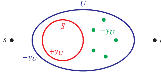
Figure 9.4 Illustration of the proof of Lemma 9.10. A set U \subseteq V \setminus \{s, t\} is shown in blue. The vertex set S of a strongly connected component of G[U] with \delta^-(S) \subseteq \delta^-(U) is shown in red. We modify our dual solution by increasing the dual variable corresponding to S , decreasing the dual variable corresponding to U (blue), and decreasing the variables corresponding to the vertices in U \setminus S (green).
