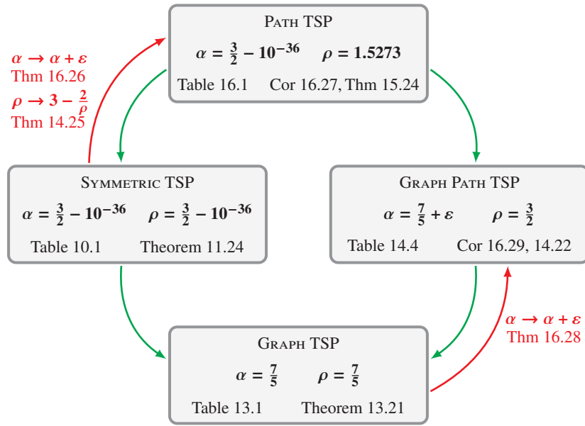
Figure 18.2 Approximation ratios ( \alpha ) and upper bounds on integrality ratios ( \rho ) for symmetric traveling salesman problems: the state of the art. An arrow from one problem to another means an approximation or integrality ratio bound for the former implies an approximation or integrality ratio bound for the latter (the same by a trivial reduction for the green arcs without labels). As lower bounds on the integrality ratios, we have \frac{4}{3} for GRAPH TSP and SYMMETRIC TSP (Proposition 2.24) and \frac{3}{2} for (GRAPH) PATH TSP (Proposition 14.15).
