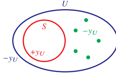
Figure 7.2 Illustration of the proof of Lemma 7.2. A nonempty set U \subseteq V is shown in blue. The vertex set S of a strongly connected component of G[U] with \delta^-(S) \subseteq \delta^-(U) is shown in red. We modify our dual solution by increasing the dual variable corresponding to S , decreasing the dual variable corresponding to U (blue), and decreasing the variables corresponding to the vertices in U \setminus S (green).
