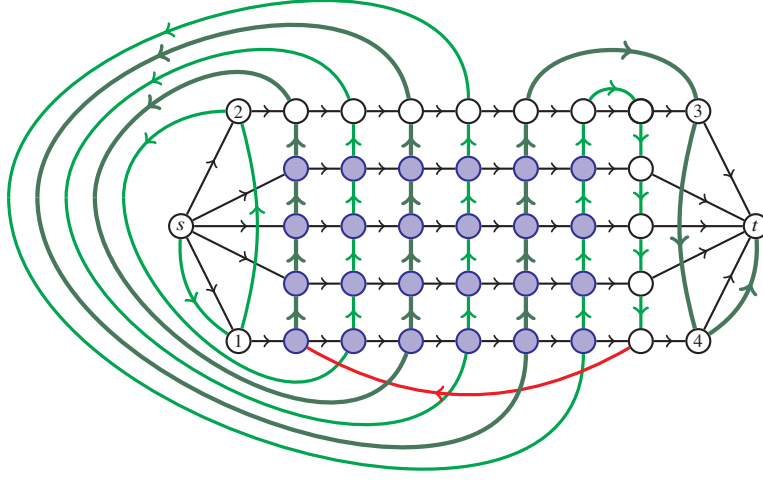
Figure 9.2 A tight example for Lemma 9.6, based on an almost tight example by Feige and Singh [2007]. The initial s - t -paths P^1, \dots, P^k are shown in black (going from left to right). A Hamiltonian s - t -path R traverses the light green edges, then the red edge, then the dark green edges. Note that the red edge is the only one that goes from right to left. The middle grid (without the vertices s, 1, 2, 3, 4, t ) has kl vertices; here, k = 5 and l = 7 . Any s - t -tour in this graph must visit s, 1, 2, 3, 4, t in this order. In between 2 and 3, it will visit the vertices in the grid in some order but must respect the order of the P^i . Our s - t -tour must use the red edge before visiting any of the (k-1)(l-1) blue vertices, and then it can visit at most k+l-3 of them before using the red edge again. Finally, after visiting the last of the blue vertices, it will visit the successor on the corresponding path P^i (in the rightmost column of the grid), and then it needs to use the red edge again in order to reach vertex 3. This makes us use the red edge at least 1 + \lceil \frac{(k-1)(l-1)}{k+l-3} \rceil times. For l \geq k^2 , this is k times. One can also see that an s - t -tour uses the red edge more than k times unless it uses almost all black edges. Therefore, if the cost of the red edge equals the total cost of the black edges, and the green edges have cost 0, the bound in Lemma 9.6 is tight (when considering the metric closure).
