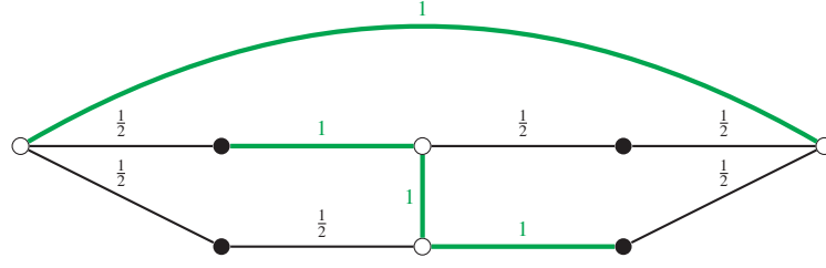
Figure 14.6 An instance of the T -TOUR PROBLEM (edge costs are not shown); T is the set of filled vertices. The numbers next to the edges show a feasible solution x^* to the LP (14.2): Thick green edges e have x_e^* = 1 , thin edges e have x_e^* = \frac{1}{2} , other edges e (not shown) have x_e^* = 0 . In fact, this is an extreme point (see Exercise 14.10). If G denotes the support graph of x^* , we see that G - T is disconnected, so G contains no spanning tree in which all elements of T are leaves (and hence G contains no spanning tree in which all elements of T have odd degree). However, \delta(t) is narrow for all t \in T , so G contains no “Gao tree.” This picture is taken from Gottschalk and Vygen [2018] (with permission from Springer Nature).
