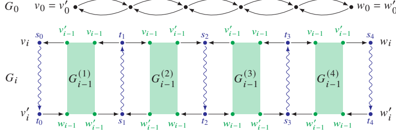
Figure 3.4 Constructing a family of digraphs with integrality ratio arbitrarily close to 2 for ASYMMETRIC TSP with unit weights. For a fixed even integer l \geq 4 , we define digraphs G_0, G_1, \dots . The digraph G_0 consists of a bidirected path of length l + 1 . Then we construct G_i from G_{i-1} as in the picture. The picture shows the construction for l = 4 ; in general, there are l copies of the graph G_{i-1} (shown in green). The blue wiggly paths indicate the paths P_i^{(j)} , each with l^i vertices. Let G'_i be the graph arising from G_i by identifying the blue v_i - v'_i -path with the blue w_i - w'_i -path. Then for i \rightarrow \infty , the integrality ratio of G'_i converges to \frac{2l}{l+1} . This picture is taken from Köhne, Traub, and Vygen [2020] (with permission from Springer Nature).
