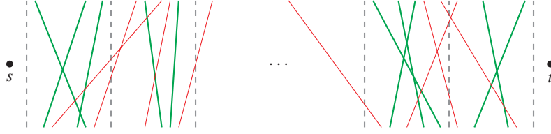
Figure 16.3 Illustration of Lemma 16.8. The dashed lines show the cuts in \mathcal{L} , which form a chain. If Q \setminus \mathcal{L} consists of the cuts sketched by the solid lines, \mathcal{B} contains the green cuts, and Q \setminus (\mathcal{B} \cup \mathcal{L}) contains the red cuts (which can be ignored if the cuts in \mathcal{L} are lonely).
