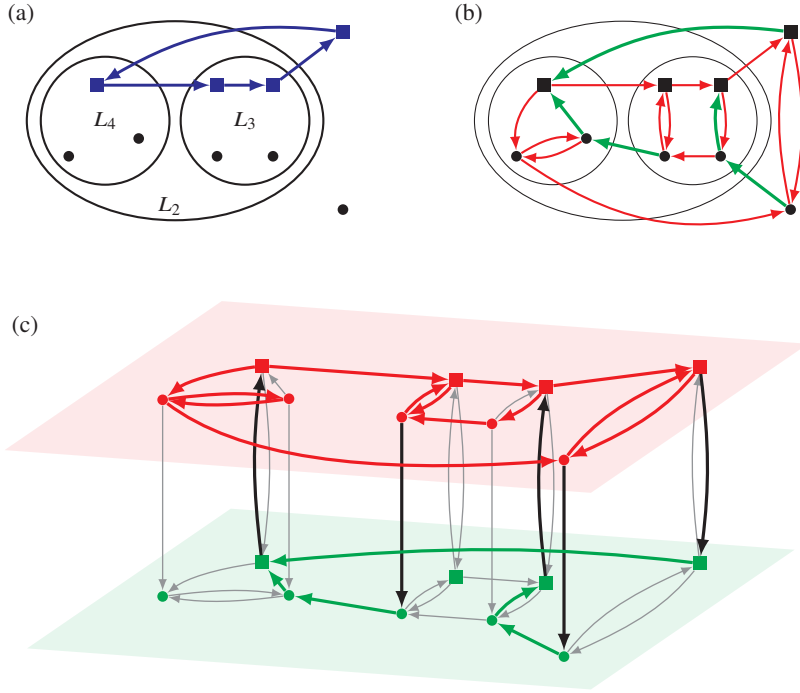
Figure 8.3 An example of the construction of the circulation z in G^{01} . Picture (a) shows the laminar family \mathcal{L}_{\geq 2} = \{L_2, L_3, L_4\} and, in blue, the backbone B . Picture (b) shows a solution x to (3.2) where we have x_e = \frac{1}{2} for all edges; a witness flow f is shown in green. The vertices in V(B) are shown as squares. Every cycle crossing the boundary of a set L \in \mathcal{L}_{\geq 2} contains both a green and a red edge. Picture (c) shows the resulting circulation z in G^{01} , where we have z_e > 0 for every thick edge e and z_e = 0 for all thin edges. The flow x - f is mapped to the upper level of the split graph (red), and the flow f is mapped to the lower level (green). This picture is taken from Traub and Vygen [2022].
