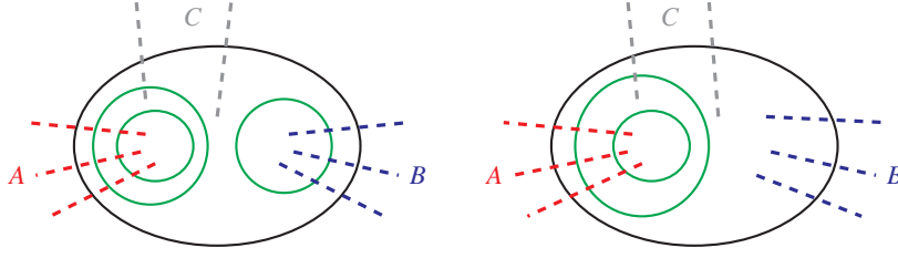
Figure 11.6 The figure shows two examples of a set W (black), the sets w \in \mathcal{H} (green) with x^*(\delta(w) \cap \delta(W)) \geq 1 - \varepsilon_{\text{partition}} and w \subseteq W . The dashed lines show the edges in \delta(W) partitioned into sets A (red), B (blue), and C (gray).
