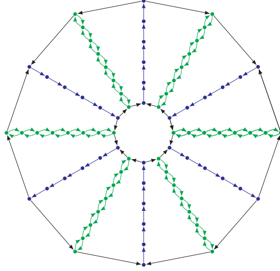
Figure 3.6 The graph G'_1 for l = 6 . An optimum LP solution has value 1 on the blue edges and value \frac{1}{2} on all other edges, and hence we have \text{LP} = |V(G'_1)| . This picture is taken from Köhne, Traub, and Vygen [2020] (with permission from Springer Nature).
