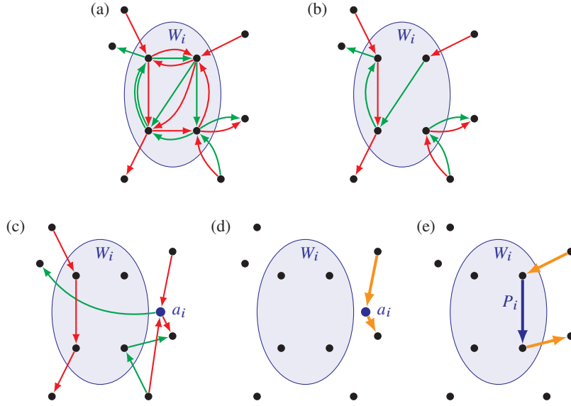
Figure 8.6 Example of the construction of the subtour cover F from the witness flow f . On all pictures, a set W_i (blue and filled) is shown. The pictures show only edges with at least one endpoint in W_i . Picture (a) shows (parts of) a possible solution x to (3.2) (green and red) and a witness flow f (green). The edges drawn with a single line have value \frac{1}{4} ; the edges drawn with a double line have value \frac{1}{2} . Recall that red edges correspond to flow on the upper level of the split graph, and green edges correspond to flow on the lower level. Picture (b) shows possible flows (\tilde{x}, \tilde{f}) = \pi(\tilde{z}) , where the circulation \tilde{z} in the split graph has acyclic support in G^{01}[W_i^{01}] . Picture (c) shows a possible circulation \tilde{x} in \tilde{G} resulting from the rerouting of flow through a_i (blue); the witness flow \tilde{f} is again shown in green. Picture (d) shows in orange a possible integral circulation \tilde{x}^* in \tilde{G} ; the orange edges are elements of the edge set \tilde{F} with \chi^{\tilde{F}} = \tilde{x}^* . Picture (e) shows the result of mapping \tilde{F} back to G . In blue, the path P_i in G[W_i] is shown; it completes the orange edges to a circulation.
