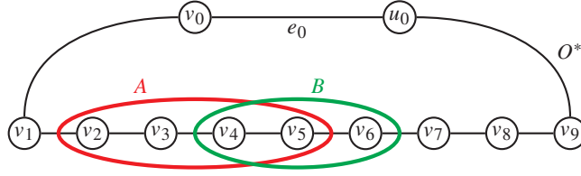
Figure 10.1 The optimum Hamiltonian cycle O^* is shown in black. Two intervals A = \{v_2, v_3, v_4, v_5\} and B = \{v_4, v_5, v_6\} are shown in red and green. A crosses B on the left.
