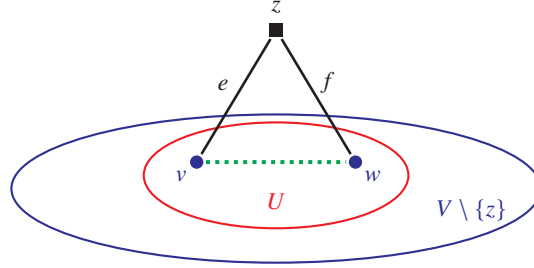
Figure 2.3 Splitting off the pair of edges e = \{v, z\} and f = \{z, w\} means replacing them by the edge \{v, w\} (green, dotted). This reduces |\delta(U)| by 2 for every set U \subseteq V \setminus \{z\} with v, w \in U (one example for such a set U is shown in red).
