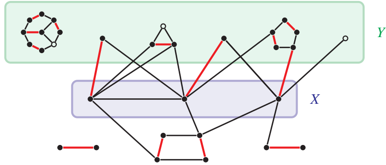
Figure 13.2 The Gallai-Edmonds decomposition of a graph G that has no perfect matching (cf. Theorem 13.6): Y contains every vertex that some maximum matching does not cover, and X is the set of neighbors of Y . The red edges form a maximum matching, covering all but three vertices (the unfilled circles in Y ).
