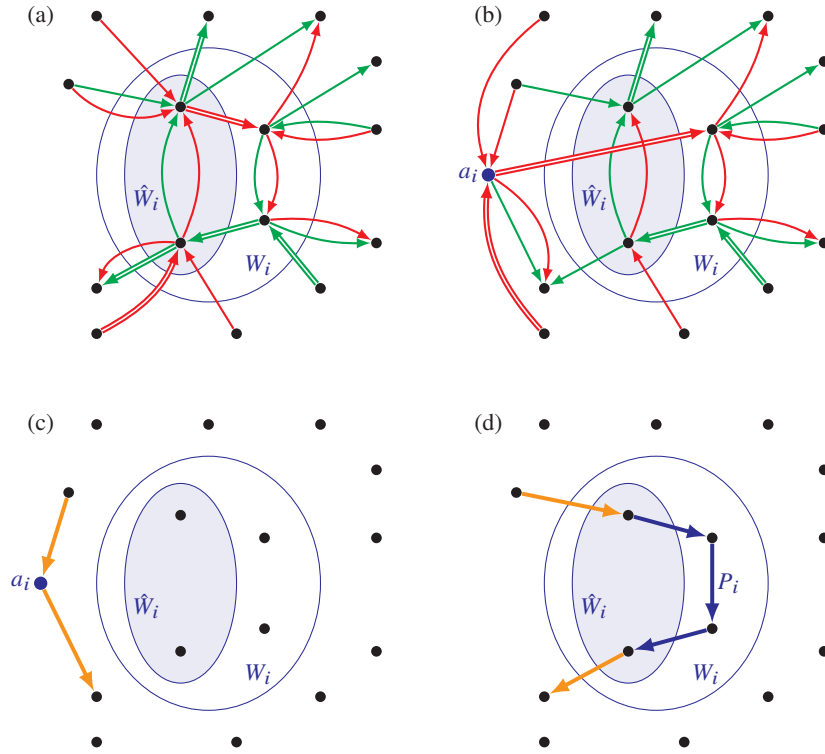
Figure 8.7 Example of the construction of the solution F from the circulation \tilde{z} in the split graph. In all pictures, a set W_i (blue with white interior) and the subset \hat{W}_i (blue and filled) is shown. The pictures show only edges with at least one endpoint in W_i . Picture (a) shows (parts of) (\tilde{x}, \tilde{f}) = \pi(\tilde{z}) where \tilde{f} (green) is a witness flow for \tilde{x} (green and red). The edges drawn with a single line have value \frac{1}{8} ; the edges drawn with a double line have value \frac{1}{4} . Note that W_i^{01} contains no high-throughput vertex. Picture (b) shows a possible flow \tilde{x} in \tilde{G} resulting from rerouting flow through a_i (blue); the witness flow \tilde{f} is shown in green. Picture (c) shows in orange a possible integral flow \tilde{x}^* in \tilde{G} . The orange edges are elements of the edge set \tilde{F} with \chi^{\tilde{F}} = \tilde{x}^* . Picture (d) shows the result of mapping \tilde{F} back to G . In blue, the path P_i in G[W_i] is shown; it completes the orange edges to a circulation. A similar picture appeared in Traub and Vygen [2022].
