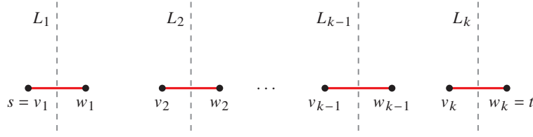
Figure 16.2 Illustration of Lemma 16.7. The dashed lines show the cuts \delta(L_i) for i = 1, \dots, k , where the sets L_i are the sets left of the dashed lines.
