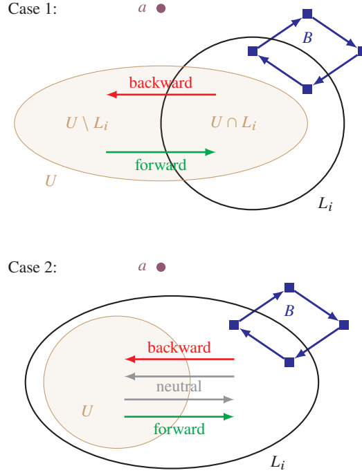
Figure 8.4 Proof of Lemma 8.7 (Case 1 and Case 2). This picture is taken from Traub and Vygen [2022].
