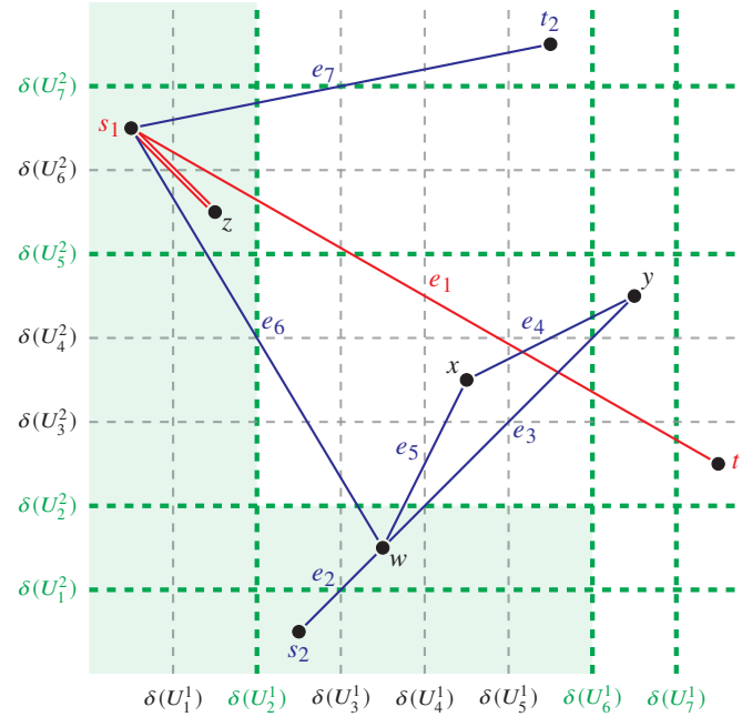
Figure 16.7 A MULTI-PATH TSP instance with eight vertices and two terminal pairs. The horizontal order corresponds to the terminal pair \{s_1, t_1\} and the vertical order to the terminal pair \{s_2, t_2\} . Suppose the red edges (F_1^*) and the blue edges (F_2^*) form an optimum solution, and let K = 3 . Then the small cuts \delta(U_j^i) (those with at most K edges in F_1^* \dot{\cup} F_2^* ) are indicated by thick green dashed lines. In this example, all edges except the two parallel red edges in the upper left are contained in a small cut.
