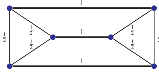
Figure 2.1 A feasible solution to the subtour LP. The value x_e is shown next to each edge e . Edges e with x_e = 0 are not shown.
