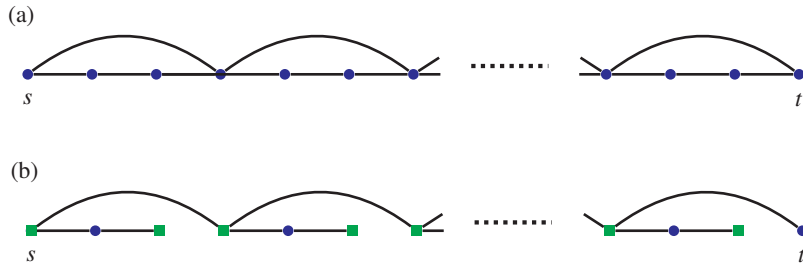
Figure 14.1 Picture (a) shows a family of examples due to Hoogeveen [1991] proving that the approximation ratio of \frac{5}{3} of Christofides' algorithm for GRAPH PATH TSP is tight. For every k \geq 1 , we have a graph with 3k + 1 vertices. Picture (b) shows a spanning tree (V, S) that might be chosen by Christofides' algorithm. The vertices with the wrong degree parity in the spanning tree (the elements of T \triangle \text{odd}(S) ) are shown as green squares. Parity correction costs 2k here.
