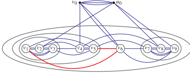
Figure 11.1 A hierarchy without polygons. Assume that the optimum tour visits v_1, \dots, v_9, u_0, v_0 in this order and the LP solution x^* puts x_e^* = \frac{1}{3} on every edge in the figure; when two or three parallel edges are drawn, the value is \frac{2}{3} or 1, respectively. In this example, the family of \eta -mincuts is laminar, shown by the ellipses in the figure (including the singletons \{v_1\}, \dots, \{v_9\} ). One can see that here none of the \eta -mincuts is irrelevant, so this laminar family is identical to the hierarchy. The thick red edges \{v_1, v_6\} and \{v_5, v_6\} both have the top cuts \{v_1, v_2, v_3, v_4, v_5\} and \{v_6\} .
