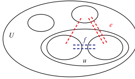
Figure 11.11 If the edge bundle e (shown in red) is bad, then e is a half-edge bundle. Because e is never reduced, the edge bundle f \in E^{\rightarrow}(u) (shown in blue) does not need to be increased in order to compensate for reductions of e .
