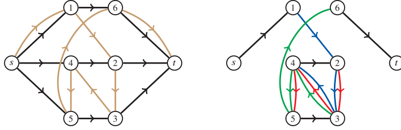
Figure 9.1 An example for the proof of Lemma 9.6. Here k = 3 . Left-hand side: The initial s - t -paths P^1, P^2, P^3 are shown in black; they go from left to right. The Hamiltonian s - t -path R (brown) visits the vertices in the order of the numbers. Right-hand side: In the proof, we combine these to a path that visits s, 1, 4, 2, 5, 3, 6, t in this order. Besides some edges of P^1, P^2, P^3 , it uses the segment from 1 to 4 from the first (blue) copy of R , the segment from 2 to 5 from the second (red) copy, and the segment from 3 to 6 from the third (green) copy.
