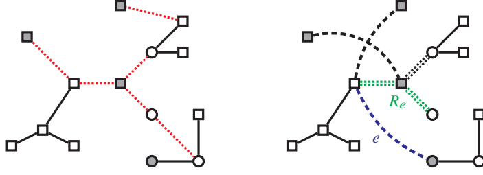
Figure 15.7 Illustration of the proof of Lemma 15.19. Vertices in T are shown as squares, other vertices as circles. On the left, we have the spanning tree (V, S) with the edges in S \setminus F_S drawn dotted and red. Filled vertices are vertices in T \triangle \text{odd}(F_S) . On the right, we have a T -tour consisting of the forest F_S (solid), a (T \triangle \text{odd}(F_S)) -join J_S (dashed), and a reconnection set R \dot{\cup} R (dotted). For the blue edge e \in J_S , the two copies of the set R_e are highlighted in green.
