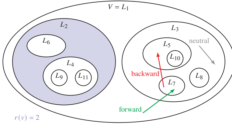
Figure 8.1 The laminar family \mathcal{L}_{\geq 2} \cup \{V\} = \{L_1, \dots, L_{11}\} . In this example, the set L_2 \setminus (L_6 \cup L_4) is the set of all vertices v with r(v) = 2 ; it is shown in blue. On the right, we see examples of a forward edge (green), a backward edge (red), and a neutral edge (gray). This picture is adapted from Traub and Vygen [2022].
