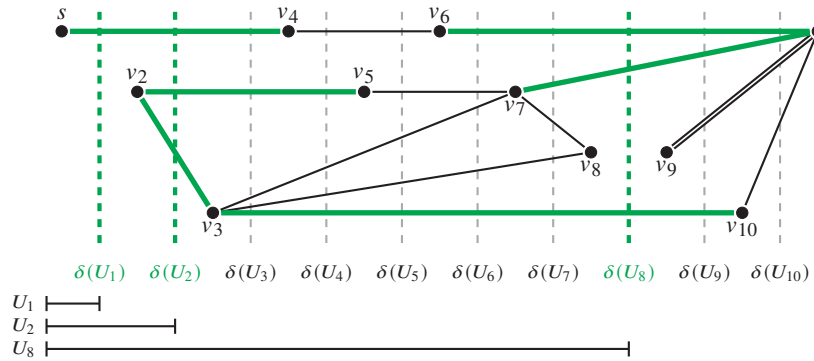
Figure 16.4 A PATH TSP instance with 10 vertices, ordered by the distance from s as in Figure 16.1. The dashed vertical lines again indicate the cuts \delta(U_j) for j = 1, \dots, n - 1 . Suppose the solid lines show the optimum \{s, t\} -tour F^* , and consider the cuts that contain at most three edges of F^* . These are the green cuts \delta(U_1) , \delta(U_2) , \delta(U_8) here, so we would try to “guess” these cuts and the bold green edges. Note that in between \delta(U_2) and \delta(U_8) , we do not have a PATH TSP instance (but a MULTI-PATH TSP instance).
