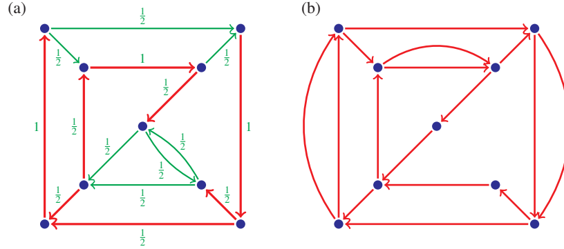
Figure 5.1 (a): A digraph G = (V, E) with a vector x \in \mathbb{R}_{\geq 0}^E . The (weakly) connected subgraph (V, R) (shown in bold red) satisfies |R \cap \delta^-(U)| \leq 2x(\delta^+(U)) for all U \subseteq V . (b): Therefore, for any cost function c , it can be extended to a tour in G that costs at most 2c(x) more than R (see Lemma 5.1). If we ignore all orientations in (a), the red tree (V, R) is 2-thin with respect to the symmetrized vector z (resulting from x as in Step (2) of Algorithm 5.4).
