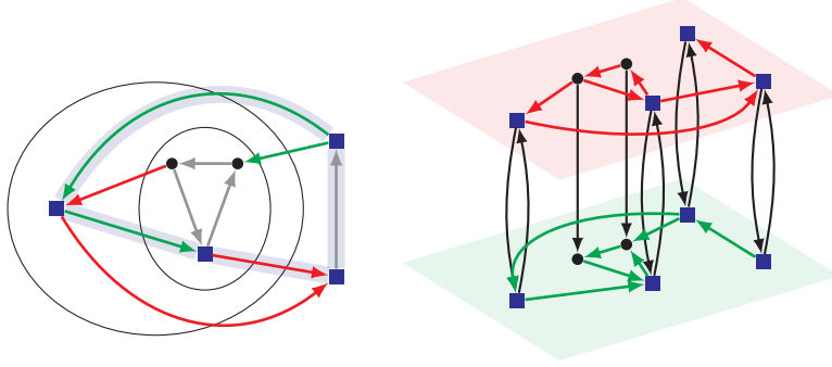
Figure 8.2 Construction of the split graph. The digraph on the left with the laminar family indicated by the two ellipses and the backbone shown in blue results in the split graph on the right (with the lower level in green and the upper level in red). Forward edges (green on the left) are mapped to the lower level, backward edges (red on the left) are mapped to the upper level. Neutral edges (gray on the left) are mapped to both levels. Additional edges (black) connect the two layers.
