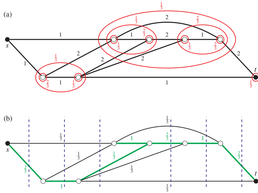
Figure 14.5 A PATH TSP instance (from Gao [2015]) with edge costs and an optimum dual solution (red ellipses) shown in (a), and with an optimum primal solution and the narrow cuts (blue, dashed) shown in (b). The green tree in (b) is the only Gao tree, and its cost is 10, more than the LP value \frac{29}{3} .
