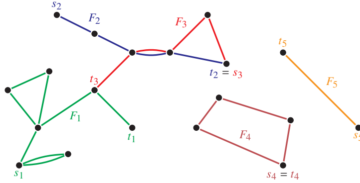
Figure 16.5 Example of a solution to a MULTI-PATH TSP instance. The different multi-edge sets F_i are shown in different colors.
