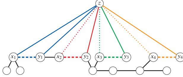
Figure 15.2 Undoing the splitting off operations at z in the proof of Lemma 15.3. Starting with the tree on the bottom (without z ), we first replace the blue dashed edge \{x_1, y_1\} by the two solid blue edges. Then, for j = 2, 3, 4 , we replace \{x_j, y_j\} by \{z, y_j\} and put the dotted edge \{x_j, z\} in the reserve list.
