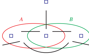
Figure 4.1 Two sets A, B \subseteq V such that A \setminus B , B \setminus A , A \cap B , and V \setminus (A \cup B) are all nonempty. The black lines indicate the six relevant types of edges.
