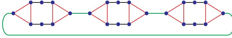
Figure 17.1 Example from Alexander, Boyd, and Elliott-Magwood [2006] showing a lower bound of \frac{6}{5} on the integrality ratio of the LP (2.12). The red edges cost 2, the black edges 1, and the green edges 0. An LP solution is given by setting x_e = \frac{1}{2} for the red edges and x_e = 1 for all other edges; its cost is 10\frac{n}{8} . Any 2-edge-connected multi-subgraph costs at least 12\frac{n}{8} .
