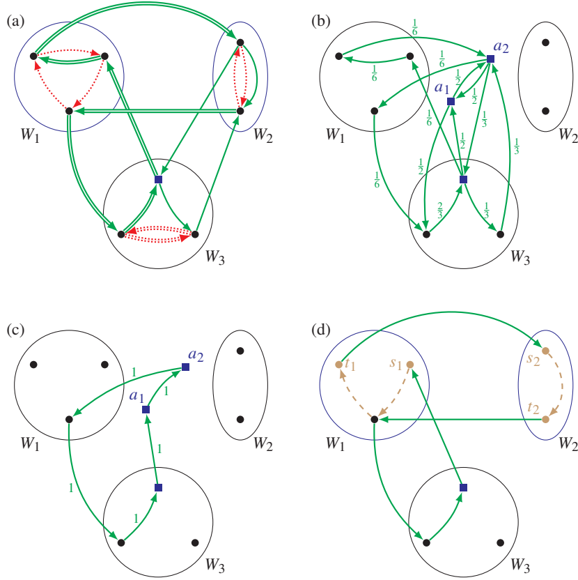
Figure 6.1 An example of the construction of a graph subtour cover (proof of Theorem 6.6). Let W_1 , W_2 , and W_3 be the vertex sets of the connected components of (V, H) ; note that H itself is not shown. (a): An LP solution x . Single edges e have x_e = \frac{1}{3} , double edges e have x_e = \frac{2}{3} . After deleting the red dotted circulation, the remaining circulation \tilde{x} (green, solid) is acyclic within each W_i . The set W_3 contains a vertex w with \tilde{x}(\delta^-(w)) \geq 1 (the blue square). (b): For the other sets, W_1 and W_2 , we reroute one unit of flow through the auxiliary vertices a_1 and a_2 , respectively. This yields the circulation \tilde{x} in \tilde{G} . (c): A possible integer circulation \bar{x}^* in \tilde{G} . (d): Mapping \bar{x}^* back to the original edges, we get the solid green edges. Together with the dashed brown paths inside W_1 and W_2 , this yields a graph subtour cover F .
