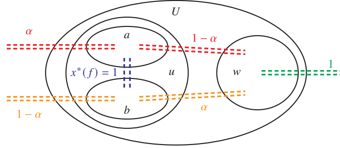
Figure 11.10 A triangle u with children a and b , where the parent U of u is also a triangle. The triangle edge bundle f = \{a, b\} is shown in blue. The edges shown in red are the edges in A^u = \delta(a) \cap \delta(u) ; the edges shown in orange are those in B^u = \delta(b) \cap \delta(u) . The edges leaving U shown on the left are those in A^U = \delta(u) \cap \delta(U) , and those edges leaving U on the right of this picture (shown in green) are those in B^U = \delta(w) \cap \delta(U) . We have x^*(A^u) \approx x^*(B^u) \approx x^*(A^U) \approx x^*(B^U) \approx 1 . For simplicity, we assume in this example that these equations are fulfilled exactly and not just approximately. Then the numbers written next to the edges denote their x^* value.
