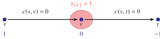
Figure 9.6 Example of an instance with LP = 0 and an optimum dual solution with a_s - a_t = 2 . The blue numbers below the vertices show the dual variables a_s = 1 , a_v = 0 , and a_t = -1 . Of course, this instance has another optimum dual solution in which all variables are zero. This picture is taken from Köhne, Traub, and Vygen [2020] (with permission from Springer Nature).
