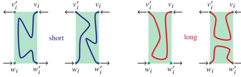
Figure 3.5 Examples of short and long visits of a subgraph G_i .
