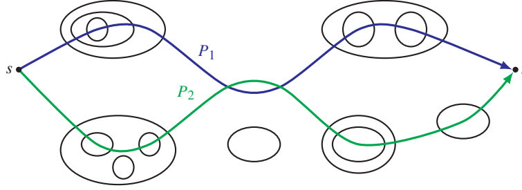
Figure 9.8 The paths P_1 and P_2 as in Lemma 9.16. In black, the vertex sets in the support of y are shown. The s - t -paths P_1 and P_2 are not necessarily internally disjoint, but they never both visit the same set U with y_U > 0 . This picture is taken from Köhne, Traub, and Vygen [2020] (with permission from Springer Nature).
