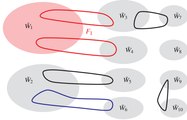
Figure 6.3 Illustration of the two possibilities for obtaining a better initialization via Lemma 6.9 when (6.12) or (6.13) is violated. Here, the filled ellipses show the partition \tilde{W}_1, \dots, \tilde{W}_{10} of V (the connected components of (V, \tilde{H}) ). The curves depict an Eulerian edge set F resulting from Theorem 6.6 for some H . (The set H is not shown here.) In blue, we see a subgraph D as in (6.13): Here D is a single connected component of (V, F) , and in this example, we have \text{ind}(D) = 2 . In red, we see a subgraph D as in Lemma 6.10: Here the red curves constitute the graph F_1 , and D is the disjoint union of E(F_1) and \tilde{H}[\tilde{W}_1] . This picture is taken from Traub and Vygen [2022].
