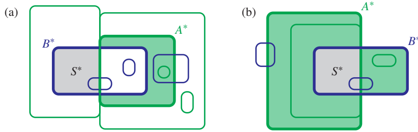
Figure 4.2 Illustration of the uncrossing procedure in the proof of Theorem 4.11. Take a maximal blue set B^* . The gray subset S^* belongs to \mathcal{U} . For every green set that crosses B^* , the intersection is either S^* or B^* \setminus S^* . (a): In Step (4) of Algorithm 4.12, we take the minimal green set A^* that crosses B^* and with B^* \setminus A^* = S^* . We uncross A^* and B^* and obtain A^* \setminus B^* and B^* \setminus A^* (the filled sets). (b): If there is no such green set, we take the maximal green set A^* that crosses B^* in Step (6). We uncross A^* and B^* and obtain A^* \cup B^* and A^* \cap B^* . New sets will be colored green.
