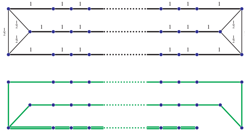
Figure 2.2 Example showing a lower bound of \frac{4}{3} on the integrality ratio of the subtour LP. The top figure shows a graph G = (V, E) , which generates the instance and which is also the support graph of an optimum solution to the subtour LP, shown by the numbers x_e ( e \in E ). The bottom figure shows an optimum tour. This is sometimes called the envelope example .
