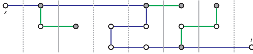
Figure 15.3 A spanning tree (V, S) . Filled circles show vertices in T \Delta \text{odd}(S) , where T = \{s, t\} . The edge set S is partitioned into its s - t -path I_S (blue) and its (\text{odd}(S) \Delta T) -join J_S (green, thick). The narrow cuts are those shown in grey (dotted and solid). Those that have an even number of edges of S are shown in solid grey; each of them contains (at least) one green and (at least) one blue edge. Three of the blue edges are lonely.
