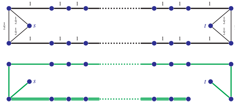
Figure 14.2 Example showing a lower bound of \frac{3}{2} on the integrality ratio of the Path TSP LP (14.1) (and hence the T -Tour LP (14.2)). The top figure shows a graph G = (V, E) with two vertices s and t . Together with c(e) = 1 for all e \in E , this defines an instance of PATH TSP. G is also the support graph of an optimum solution to the LP (14.1) in the metric closure, shown by the numbers x_e ( e \in E ) in the top figure. The bottom figure shows an optimum \{s, t\} -tour.
