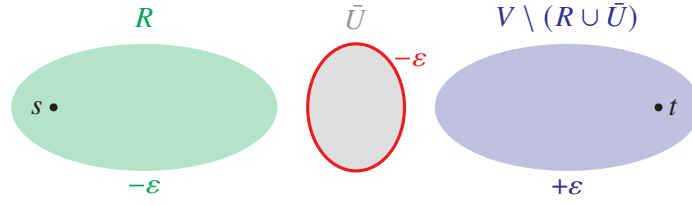
Figure 9.7 Modifying the dual solution in the proof of Lemma 9.14. The green and blue numbers in the bottom indicate the change of the dual variables corresponding to the vertices. In red, the decrease of the variable y_{\bar{U}} is indicated. There is no edge from R to V \setminus (R \cup \bar{U}) . This picture is taken from Köhne, Traub, and Vygen [2020] (with permission from Springer Nature).
