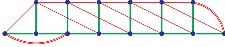
Figure 17.2 Example from Cheriyan et al. [2008] showing a lower bound of \frac{3}{2} on the integrality ratio of the LP that results from (2.12) by adding the constraints x_e \leq 1 for all e \in E . We have 2k + 2 vertices (here k = 6 ). The 2k + 1 green edges have cost 0, and the red edges have cost 1. Setting x_e = 1 for the green edges, x_e = \frac{1}{3} for the single red edges, and x_e = \frac{2}{3} for the two bent double red edges yields a feasible LP solution of total cost \frac{2}{3}k + 1 . There is no simple 2-edge-connected spanning subgraph with fewer than k + 1 red edges. Since there is a spanning tree of cost 0, this is actually an instance of the tree augmentation problem.
