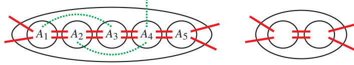
Figure 11.8 A polygon (here with atoms A_1, \dots, A_5 ) looks like the picture on the left. Every pair of parallel red edges stands for a set of edges with total x^* value very close to 1. Other edges e (like those shown in green, dotted) may exist, but with x_e^* very small. Therefore, a polygon behaves like a triangle (shown on the right).
