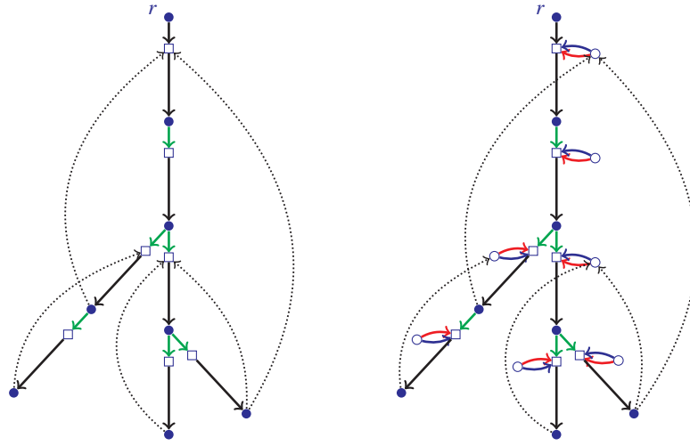
Figure 12.4 For the DFS tree in Figure 12.3, the left-hand side shows the constructed flow network (D, l) in which we look for a circulation f with minimum cost \text{cost}(f) . New vertices z_e ( e \in S ) are shown as squares. Green arcs require at least one unit of flow. The right-hand side shows how to transform this to an equivalent standard minimum-cost circulation problem. Blue arcs can carry at most one unit of flow. Red arcs have cost 1; all other arcs have cost 0.
