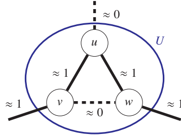
Figure 11.4 Suppose U \in \mathcal{H} has exactly three children u , v , and w and x^*(\delta^\uparrow(u)) \approx 0 . Then x^*(\delta^\uparrow(v)) \approx 1 and x^*(\delta^\uparrow(w)) \approx 1 . Moreover, x_{\{u,v\}}^* \approx 1 and x_{\{u,w\}}^* \approx 1 .
