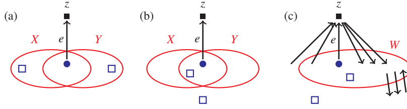
Figure 3.2 (a) and (b): The two cases in the proof of (3.4). (c): The maximal dangerous set W : Assuming \delta^+(z) \subseteq \delta^-(W) leads to a contradiction. The blue empty squares indicate elements of T .
