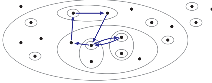
Figure 7.6 Example of a vertebrate pair (I, B) . The laminar family \mathcal{L} of I is shown in gray, and a backbone B is shown in blue. The edges of G are not shown. This picture is taken from Traub and Vygen [2022].
