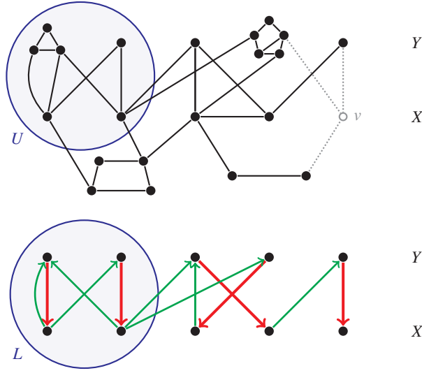
Figure 13.3 Top: The Gallai–Edmonds decomposition of G' = G - v in the proof of Theorem 13.9. Bottom: The digraph D . The red, thick edges oriented from Y to X belong to M . The graph L is a strongly connected component of D without entering arcs, and U is the corresponding vertex set in G .
