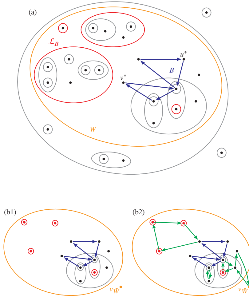
Figure 7.7 Illustration of Algorithm 7.8. The ellipses show the laminar family \mathcal{L} . Picture (a) shows the set W (orange), the subtour B (blue), and the elements of \mathcal{L}_{\bar{B}} (red). The subtour B is the union of the paths P_{u^*, v^*} and P_{v^*, u^*} . Picture (b1) shows the resulting vertex pair as constructed in Step (2) of Algorithm 7.8. The vertices resulting from the contraction of elements of \mathcal{L}_{\bar{B}} are shown in red, and the vertex v_W that results from the contraction of V \setminus W is shown in orange. Picture (b2) shows in green a possible solution to this vertex pair as computed in Step (3). Step (4) of Algorithm 7.8 is illustrated by Figure 7.8. This picture is taken from Traub and Vygen [2022].
