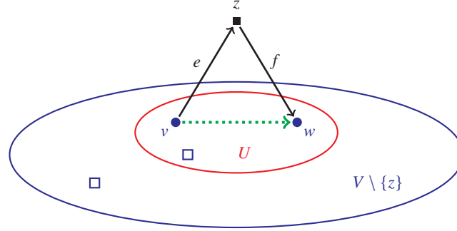
Figure 3.1 Splitting off the pair of edges e = (v, z) and f = (z, w) means replacing them with the edge (v, w) (green, dotted). This reduces |\delta(U)| by 2 for every set U \subseteq V \setminus \{z\} with v, w \in U . For sets U with |\delta(U)| = \lambda and T \cap U \neq \emptyset and T \setminus U \neq \emptyset , this would lead to violating (3.3). One example for such a set U is shown in red; here, the blue empty squares indicate elements of T .
