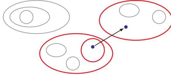
Figure 7.3 Structure of the cost function c^y induced by a strongly laminar ASYMMETRIC TSP instance. The cost of the edge e shown in black is the sum of the values y_U for the sets U \in \mathcal{L} with e \in \delta(U) ; these elements of the laminar family \mathcal{L} are shown in red.
