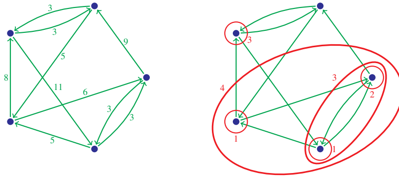
Figure 7.4 An example of a cost function (left) induced by a vector y whose support is a laminar family of vertex sets (right).
