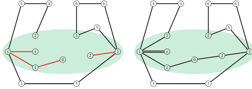
Figure 13.6 Illustrating the algorithm described in the proof of Lemma 13.20, continuing the example from Figure 13.5. Left: The edges of pendant ears after optimizing short ears (black) and a minimal set of edges of non-pendant ears (red) to make a connected spanning subgraph. Right: For correcting parities (in the green subgraph G[V \setminus V_\pi] ), we need three more edges; a possible resulting tour is shown.
