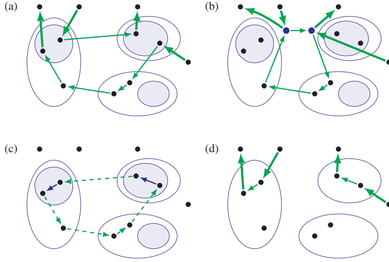
Figure 8.8 Illustration of the proof of Lemma 8.20. Three sets W_i are shown in blue with white interior; pictures (a)–(c) also show their subsets \hat{W}_i (blue and filled). Picture (a) shows (parts of) an arbitrary witness flow f (green). The thin edges are neutral; the thick edges can be neutral or forward edges. This witness flow f will not be chosen by our algorithm; it does not minimize \sum_{i=1}^q f(\delta(W_i)) . Picture (b) shows what would happen if we chose this flow anyway. We see a possible result of rerouting this flow through the vertices a_i \in V(\bar{G}) (shown in blue). In this example, the support of \bar{f} contains a cycle \bar{C} . Picture (c) shows a corresponding closed walk C in the residual graph G_f . The blue edges show paths inside the sets \hat{W}_i ; these exist because G_f[\hat{W}_i] is strongly connected. Picture (d) shows the flow resulting from f by augmenting along C . The augmentation decreased \sum_{i=1}^q f(\delta(W_i)) but did not change the flow on forward edges. This picture is taken from Traub and Vygen [2022].
