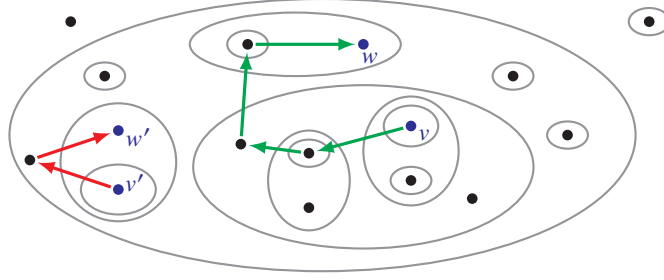
Figure 7.5 A nice path from v to w is shown in green. The laminar family \mathcal{L} is shown in gray. The edges of G are not shown. The red path from v' to w' is not nice because it re-enters a set from \mathcal{L} that it has previously left.
