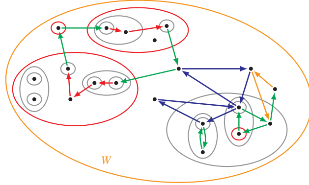
Figure 7.8 Illustration of Step (4) of Algorithm 7.8, continuing Figure 7.7. The green edges are those that arise from the vertebrate pair solution from Figure 7.7 (b2) by undoing the contraction of the sets in \mathcal{L}_B . The red edges are the paths that we add to connect within L \in \mathcal{L}_B when uncontracting L . The orange edges show the u - v -path in G[W] that we add to replace the edges (u, v_W) and (v_W, v) in the vertebrate pair solution from Figure 7.7 (b2). This picture is taken from Traub and Vygen [2022].
