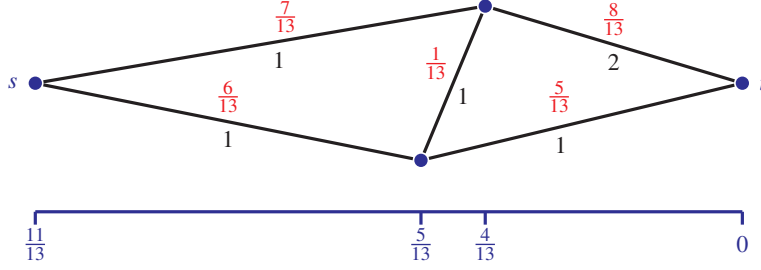
Figure 5.3 A small electrical network (with \lambda_e shown in black below every edge e ). The electrical s - t -flow of value 1 is shown in red above the edges, flowing from left to right. A corresponding potential \pi is shown in blue below.
