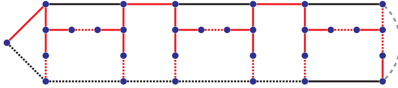
Figure 13.7 Example showing that the tour computed by the algorithm of Theorem 13.21 is not necessarily much shorter than \frac{7}{5} times the optimum. For every k \in \mathbb{N} , we have a Hamiltonian graph with 10k + 1 vertices and 13k + 1 edges. The figure shows the case k = 3 . A nice open ear-decomposition starts with 2k ears of length 5 from left to right, each with three vertical edges, and then proceeds with k horizontal pendant 3-ears and one trivial ear (the dashed edge on the right). Here \pi = k = \frac{1}{10} \Lambda(G, \mathcal{I}) , but no matter whether we apply Theorem 13.4 (if dotted edges are removable) or Lemma 13.20 (if the red edges form the spanning tree), we can end up with 14k edges. This picture is adapted from Sebő and Vygen [2014] (with permission from Springer Nature).
