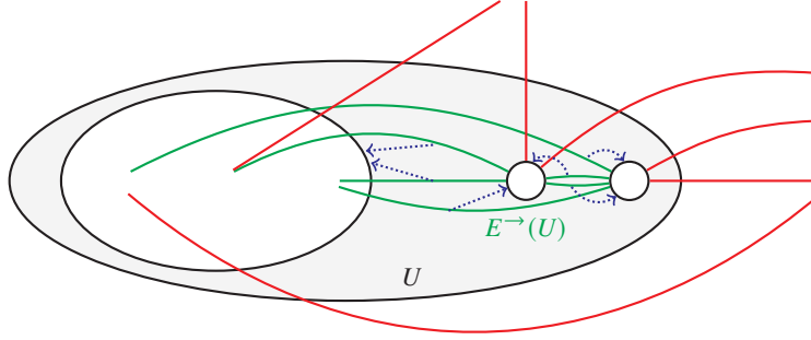
Figure 11.3 A set U \in \mathcal{H} (the large ellipse, corresponding to \{v_1, \dots, v_5\} in Figure 11.1) with its three children. The edges in E^{\rightarrow}(U) are shown in green; the edges in \delta(U) are shown in red. The dotted blue arrows show a possible assignment of the green edges to the vertices: In this case, each green edge pays for exactly one incident red edge. In general, the assignment can be fractional.
