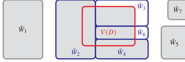
Figure 6.2 Illustration of the proof of Lemma 6.9. The gray and blue rectangles show the partition of V into \tilde{W}_1, \dots, \tilde{W}_7 . In red, we see the vertex set V(D) of the given connected graph D with \text{ind}(D) = 2 . The rectangles with blue boundaries show the sets \tilde{W}_i with i \in I . In this example, I = \{2, 3, 4, 6\} . The filled areas show vertex sets of connected components of (V, \tilde{H}') . In this example, we have J = \{2, 4\} . The connected components \tilde{H}[\tilde{W}_1] , \tilde{H}[\tilde{W}_5] , and \tilde{H}[\tilde{W}_7] remain unchanged, and we get a new component D^* with vertex set V(D) \cup \tilde{W}_2 \cup \tilde{W}_4 ; we also get singleton components (without edges) for all vertices in \tilde{W}_3 \setminus V(D) and \tilde{W}_6 \setminus V(D) . This picture is taken from Traub and Vygen [2022].
