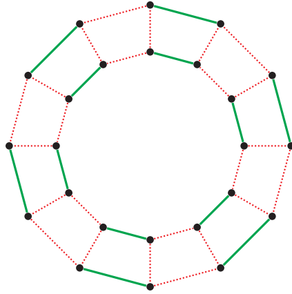
Figure 10.3 A donut graph (for k = 6 ). Consider the LP solution x^* with x_e^* = 1 for every solid green edge e and x_e^* = \frac{1}{2} for every dotted red edge e .
