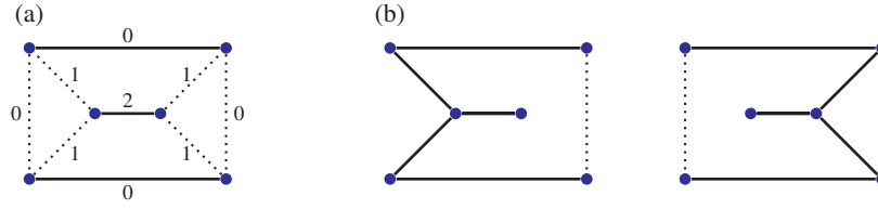
Figure 15.1 Example due to Schalekamp and van Zuylen, proving that for the SYMMETRIC TSP, the Best-of-Many Christofides algorithm does not have a better approximation ratio than \frac{3}{2} . The numbers next to the edges in (a) denote their cost. In an optimum LP solution, the dotted edges in (a) have value \frac{1}{2} and the solid edges have value 1. The LP value is 4. (b) shows a decomposition of the optimum LP solution into two spanning trees (each with weight \frac{1}{2} ) plus the dotted edges. Both spanning trees cost 4, and for both of them, parity correction costs 2.
